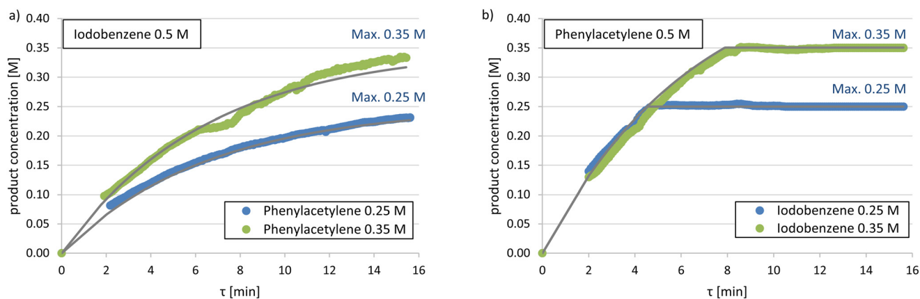
Fig. 7 Product concentration profiles at varying initial concentrations of a) phenylacetylene with constant initial concentration of iodobenzene (0.5 mol L -1 ) and b) iodobenzene with constant initial concentration of phenylacetylene (0.5 mol L -1 ). Reaction conditions: Pd(PPh 3 ) 4 (0.0025 M), CuI (0.005 M), NEt 3 (1.5 M), 90 °C.
